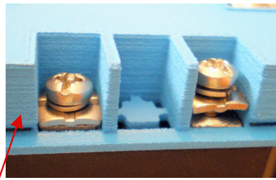
Connexions de commande M4 M4 control connections
