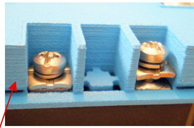
M4 control connection
