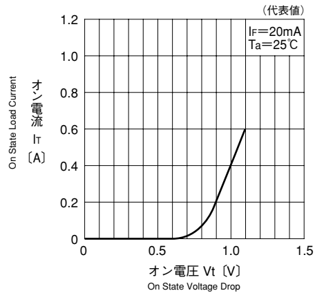
On State Load Current VS. On State Voltage Drop
